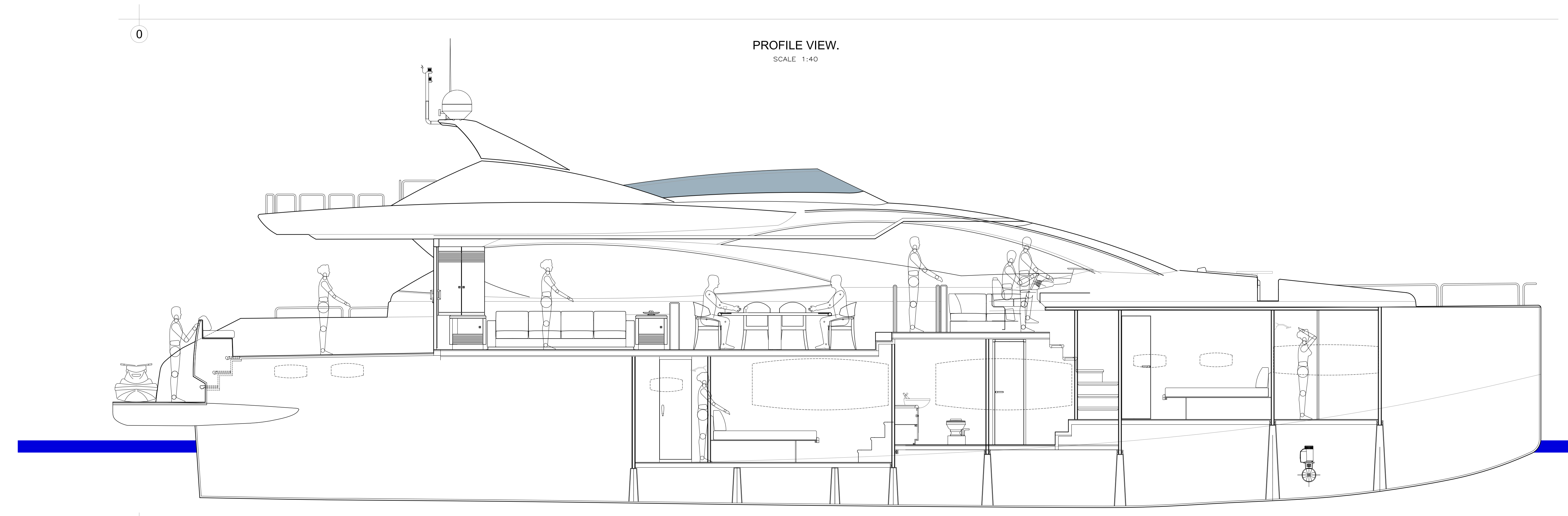
LONGITUDINAL SECTION. SCALE 1:40
