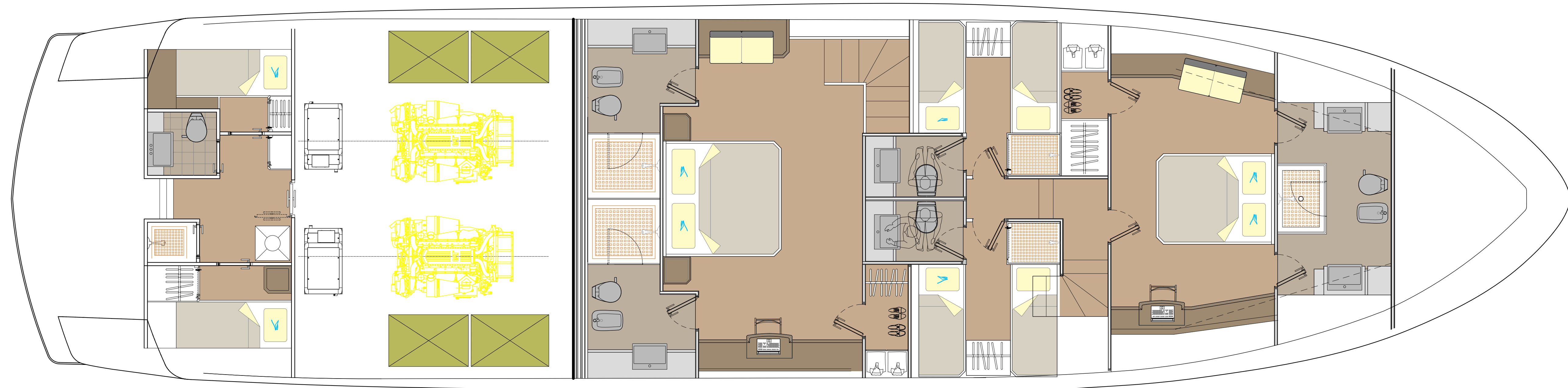
INTERIOR TOP VIEW. SCALE 1:40
