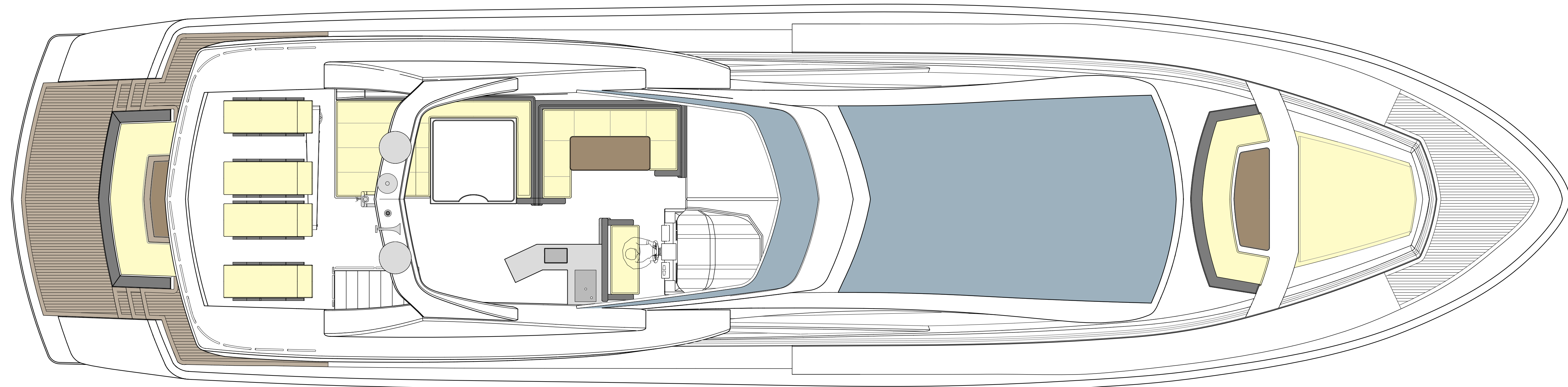
FLYBRIDGE TOP VIEW. SCALE 1:40
