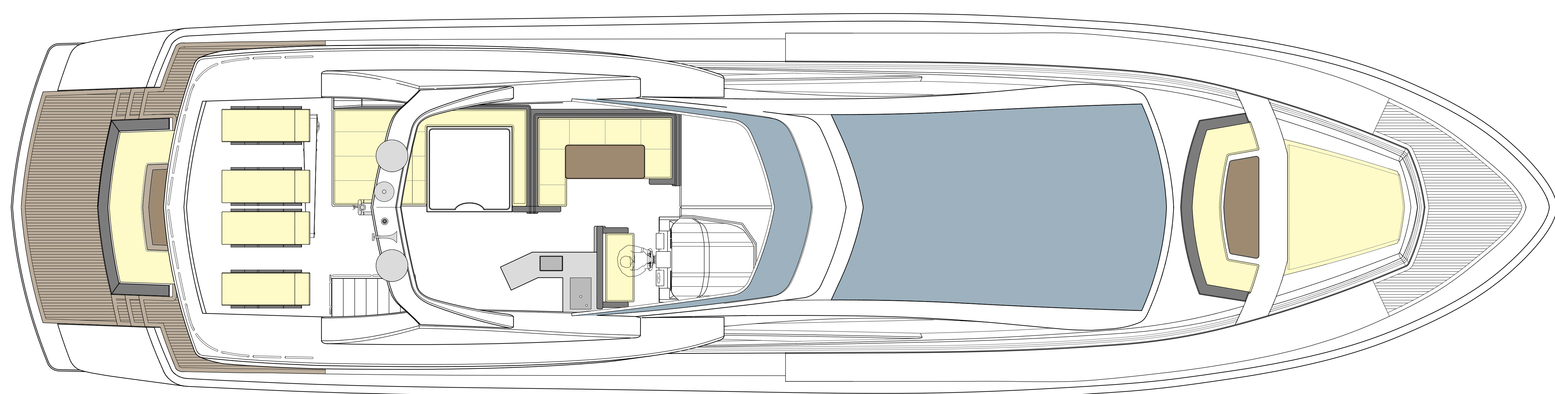
FLYBRIDGE TOP VIEW. SCALE 1:40
